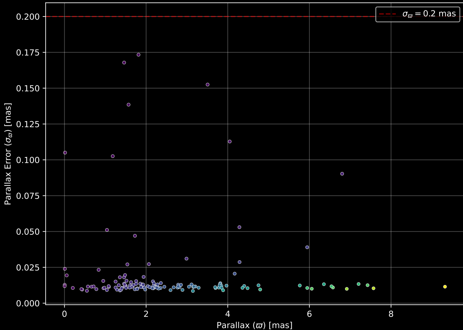
GALAH DR4 Field: [7177] Parallax Quality (n= 130)
