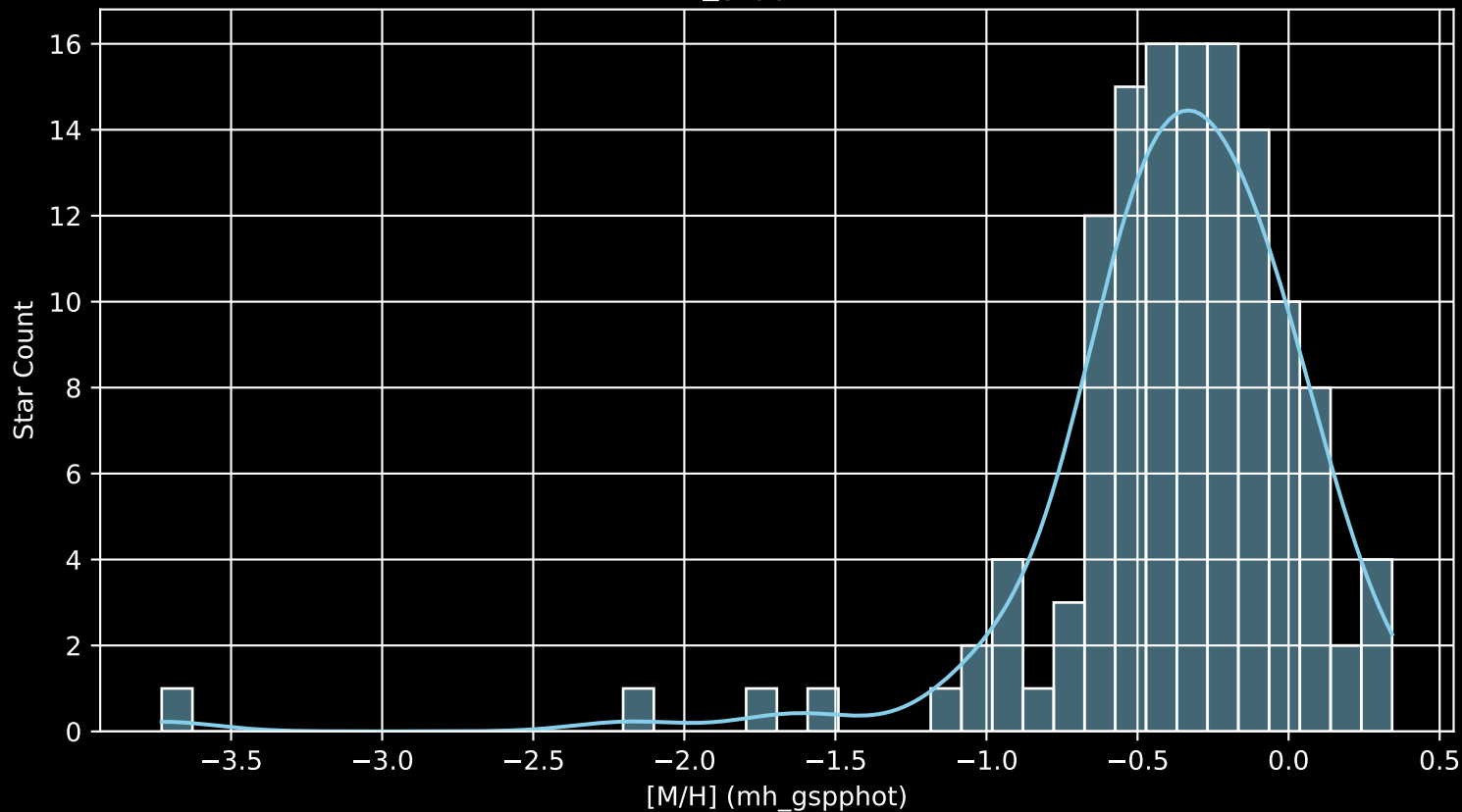
GALAH DR4 Field: [7177] [M/H] (mh_gspphot) (n= 128)
