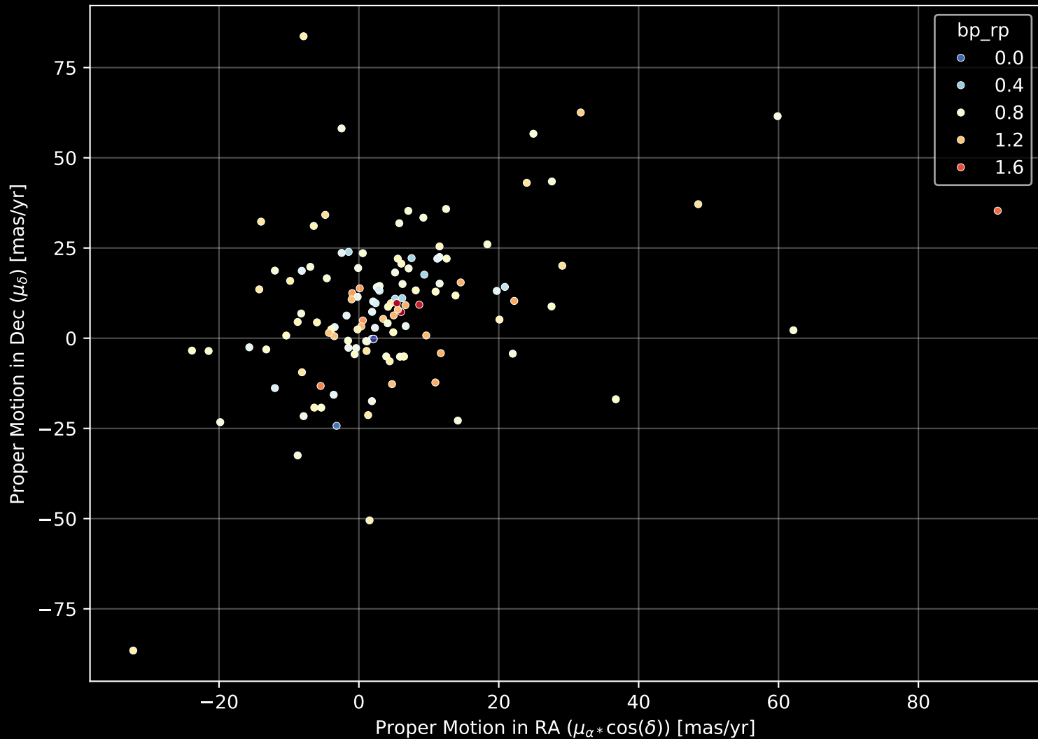
GALAH DR4 Field: [7177] Proper Motion Diagram (n= 130)
