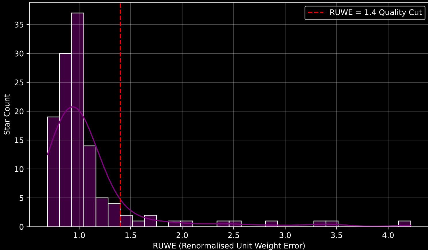
GALAH DR4 Field [7177] RUWE Distribution (n= 122)
