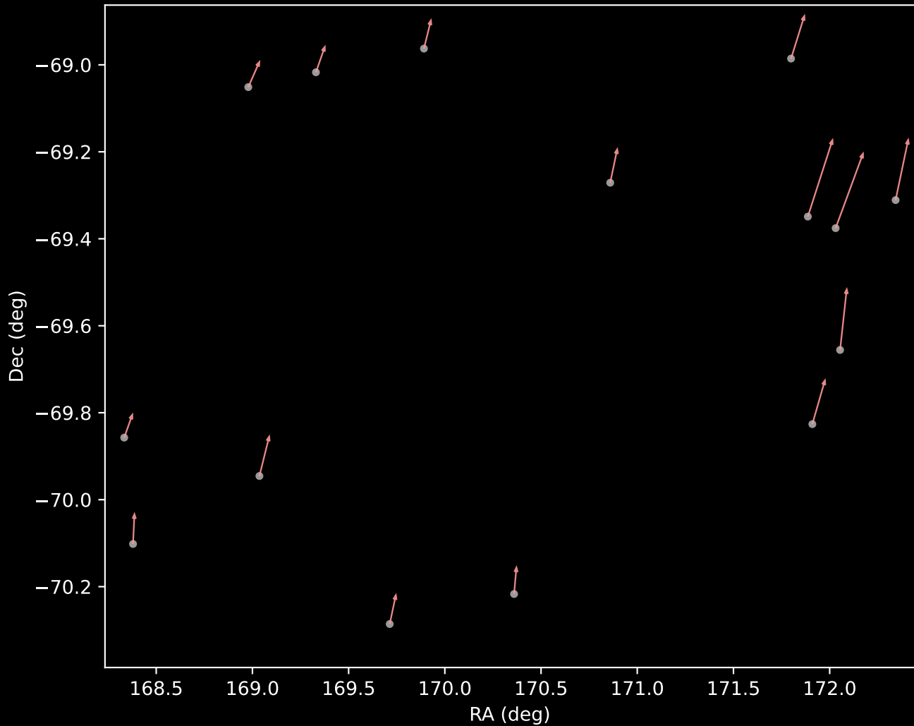
GALAH DR4 Cluster 7 Proper Motion Vectors (n=15)
