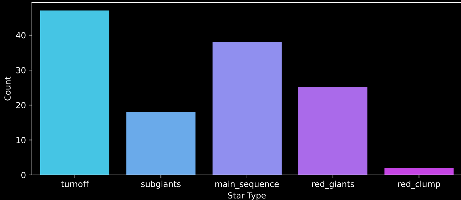
GALAH DR4 Field: [7177] Count plot of Star Type
